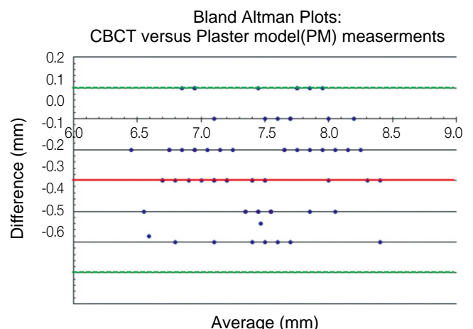
Fig. 2. Bland-Altman plots comparing plaster model(PM) and CBCT measurements. The red line is the mean difference line. The green lines represent the mean difference \pm 2 SD.
