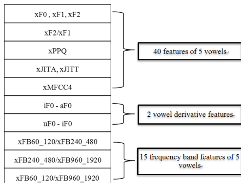
Figure 3. Voice features of 5 vowels
