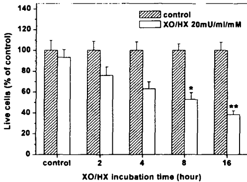
Fig. 2. Time-dependency of Xanthine Oxidase(XO) and Hypoxanthine(HX) in cultured mouse spinal sensory neurons.
