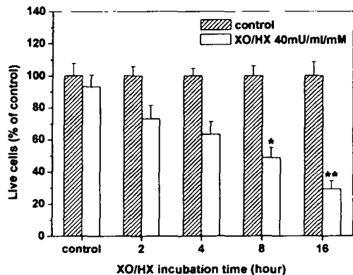
Fig. 4. Time-dependency of Xanthine Oxidase(XO) and Hypoxanthine(HX) in cultured mouse spinal sensory neurons.
