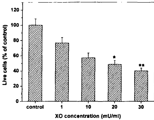
Fig. 1. Dose-dependency of Xanthine Oxidase(XO).
