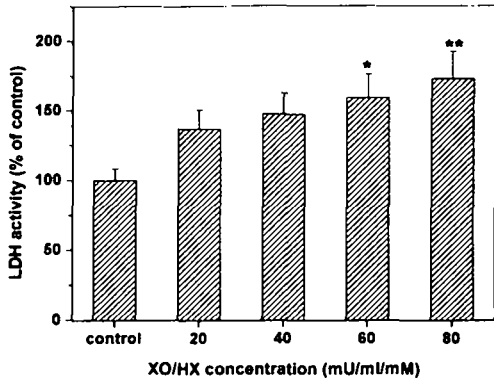
Fig. 7. Dose-dependency of Xanthine Oxidase(XO) and Hypoxanthine(HX).
