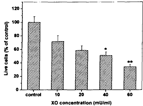
Fig. 3. Dose-response relationship of Xanthine Oxidase(XO) in cultured mouse spinal sensory neurons.
