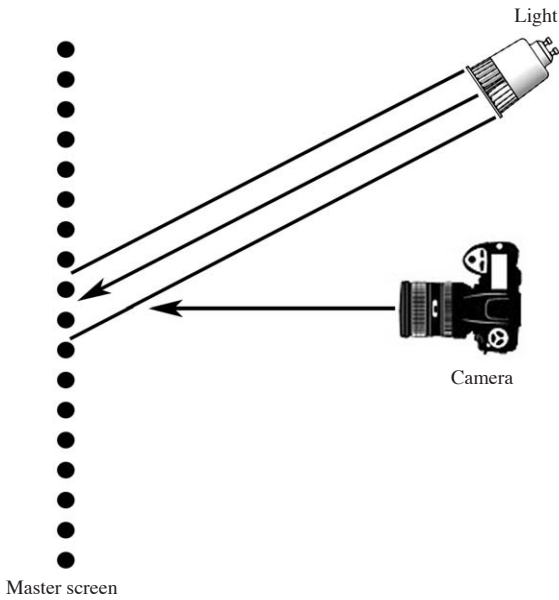
Fig. 2. Diagram illustrate the schematic position for light and camera toward the master screen. The angle between light source and camera is 65°, and the distance between camera and master screen is 1.2m.
