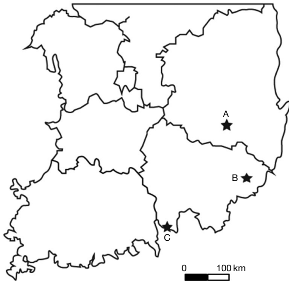
Fig. 1. Geographical location of Nukdo, Imdang, Yeanri site. A: Imdang, B: Yeanri, C: Nukdo
