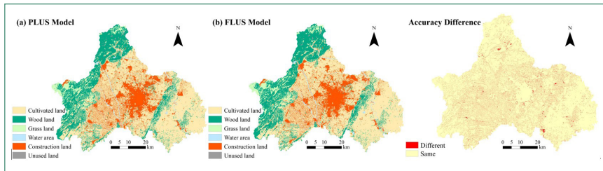
Figure 6 Variations in model accuracy in Chengdu
