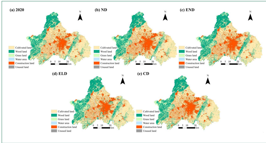
Figure 10 Spatial distribution of landscape types under multi-scenarios in Chengdu
