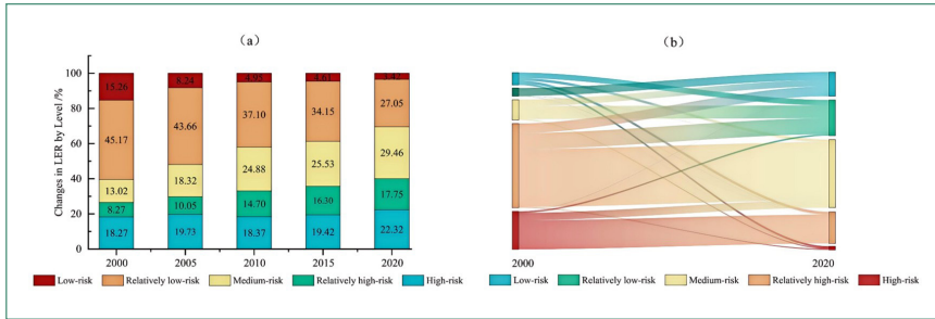
Figure 2 Change in LER in Chengdu
