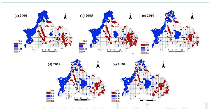
Figure 4 LISA Cluster Analysis of LER
