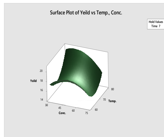
Fig. 4. Surface plot of Yield v/s Temperature and Concentration
