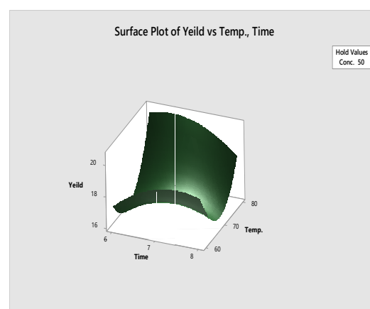
Fig. 5. Surface plot of Yield v/s Temperature and Time
