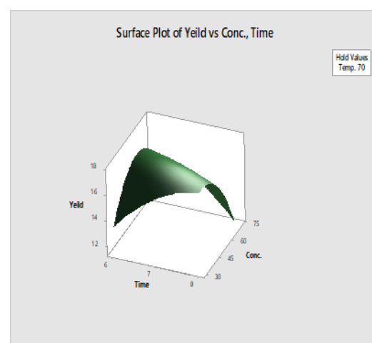
Fig. 6. Surface plot of Yield v/s Concentration and Time
