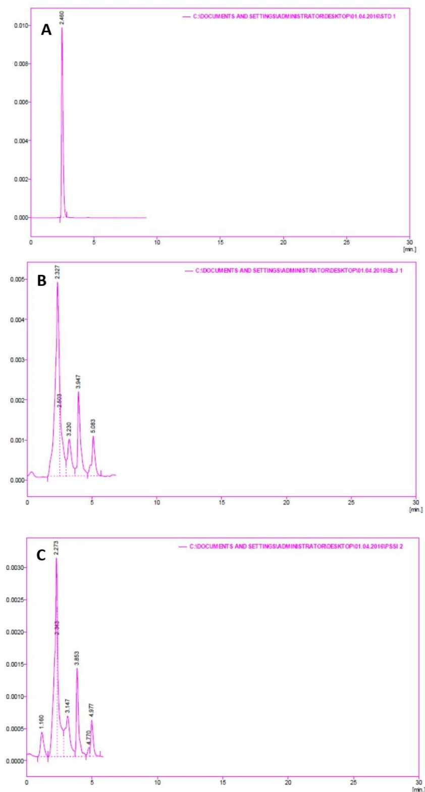
Fig 3. Total alkaloid analysis of (A) standard atropine, (B) baseline sample of and (C) light challenged sample of using HPLC
