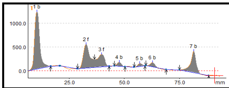
Fig.4 Densitogram of alcoholic extract of Qurş-e-Mafasil upon derivatized with vanillin sulfuric acid reagent at \lambda 580 nm.
