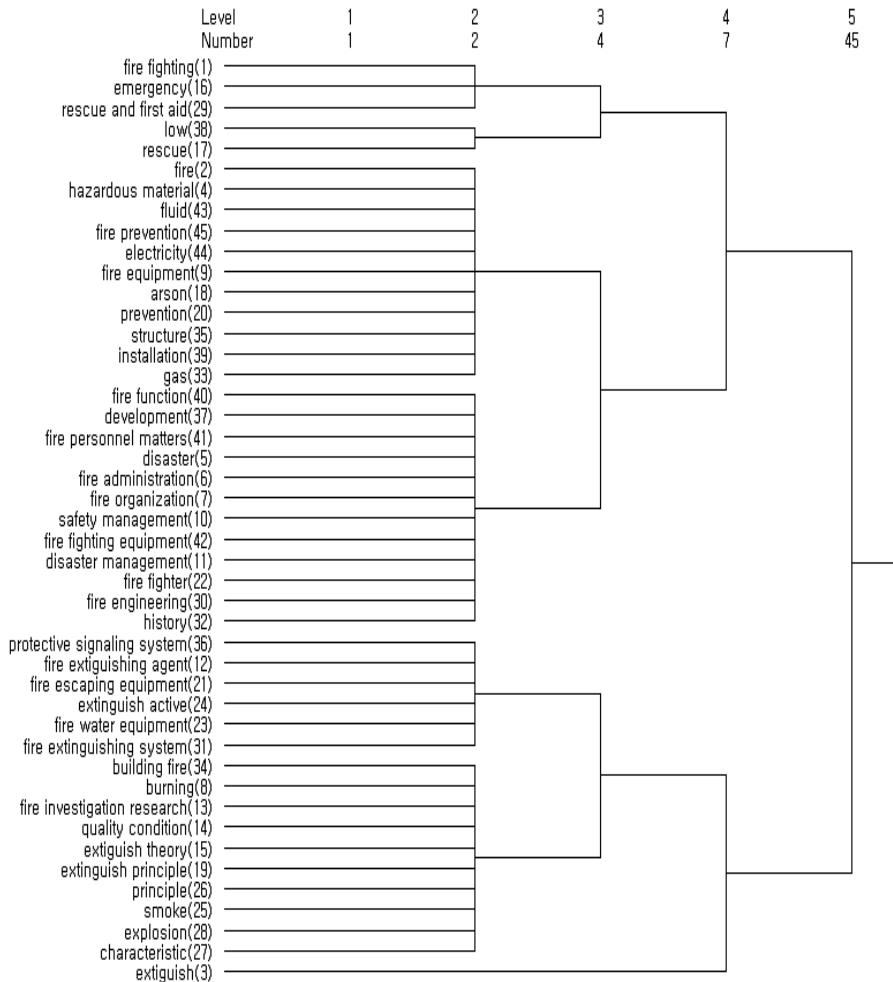
<Fig 1> Dendrogram by Structural Equivalence Analysis
