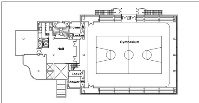
[Figure 6] Type A-3 Plan (PS14 Sports Center)
