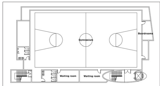
[Figure 4] Type A-1 Plan (PS16 Sports Center)
