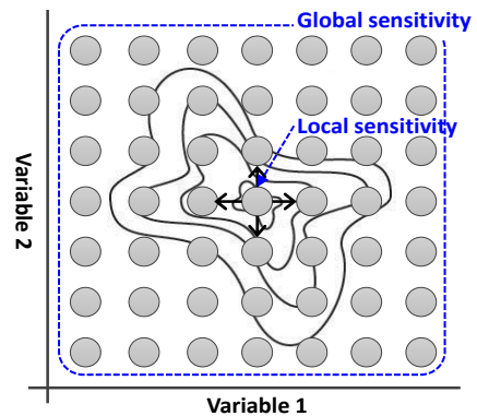
[Figure 4] Difference between local and global sensitivity
