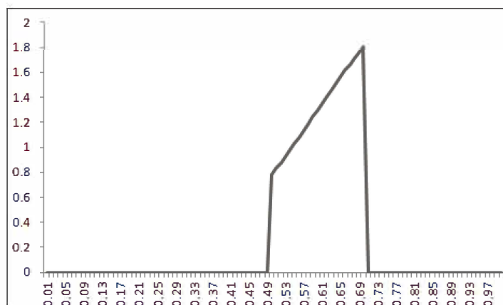
Figure 1. Post-distribution of coins
