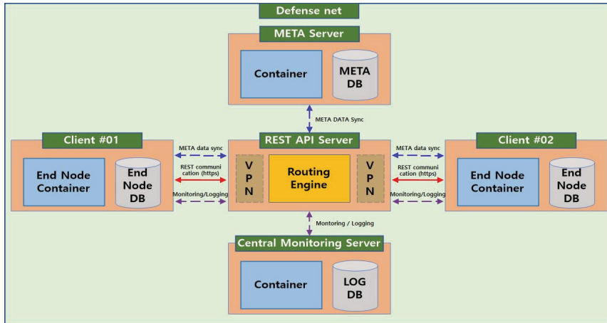
&lt;Figure 6&gt; Defense REST API Server Reference Model
