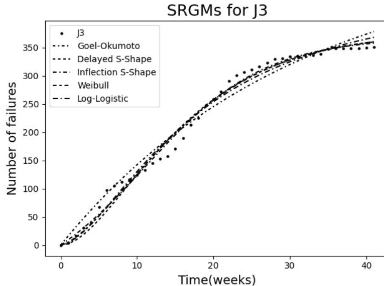
〈Figure 5〉 Graph of SRGMs with minimum MSE for J3
