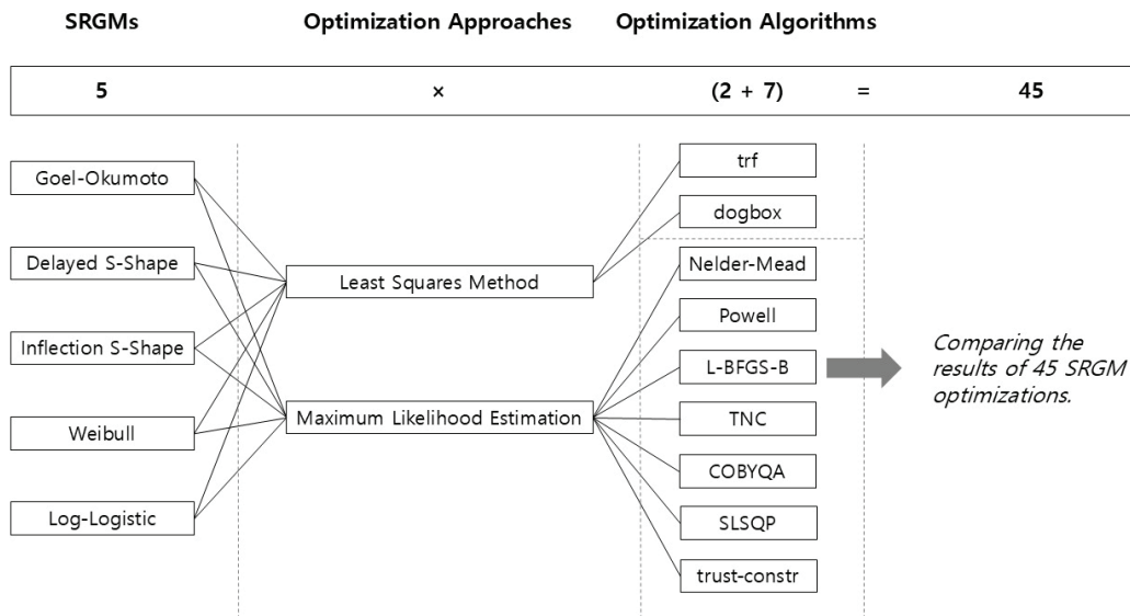
〈Figure 2〉 Optimization process of SRGMs (Software Reliability Growth Models)
