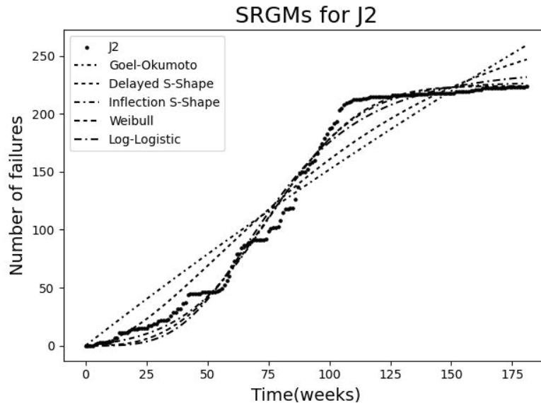
〈Figure 4〉 Graph of SRGMs with minimum MSE for J2
