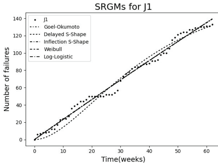
〈Figure 3〉 Graph of SRGMs with minimum MSE for J1
