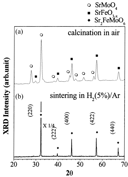
Fig. 2. XRD data of SFMO pellet (a) after calcination in air at 900°C and (b) after sintering in H 2 (5%)/Ar at 1150°C.
