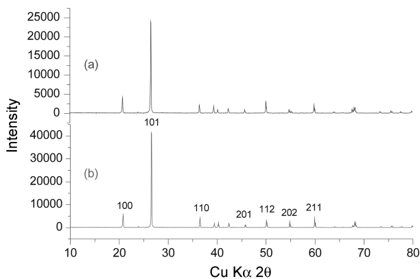
Fig. 7. X-ray patterns of natural Zambian amethyst. (a) non-treated natural Zambian amethyst, (b) natural Zambian amethyst treated hydrothermally at 300°C for 30 hrs in HCl.
