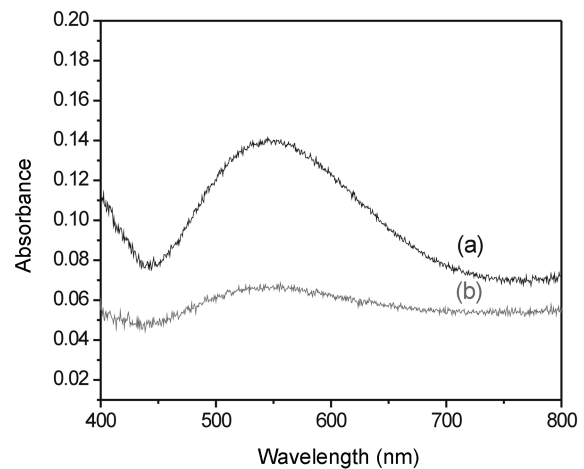
Fig. 6. The result of optical curves for natural Zambian amethyst. (a) non-treated natural Zambian amethyst, (b) natural Zambian amethyst treated hydrothermally at 300°C for 30 hrs in HCl.
