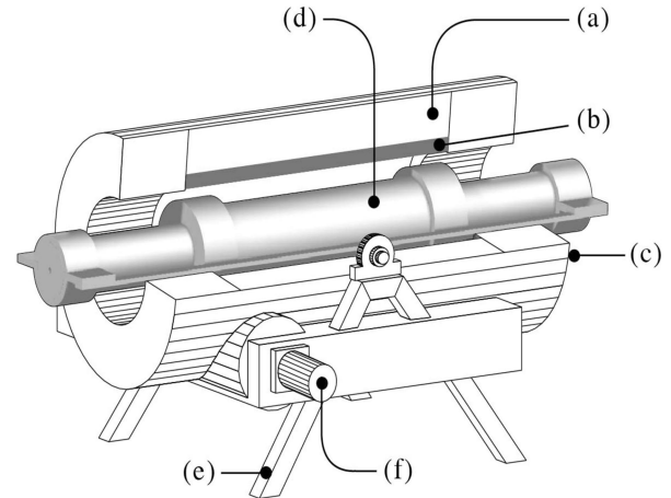
Fig. 2. A schematic diagram of apparatus used for hydrothermal treatment of natural Zambian amethyst. (a) insulator, (b) electric heater, (c) furnace, (d) autoclave, (e) susceptor, (f) motor.
