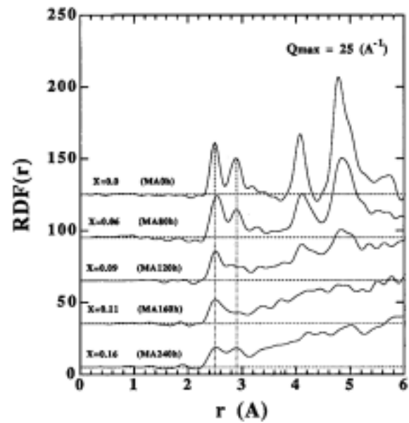
Fig. 8. Neutron radial distribution functions RDF(r) for (V_{70}Fe_{30})_{1-x}N_x powders as a function of the absorbed nitrogen concentration.
