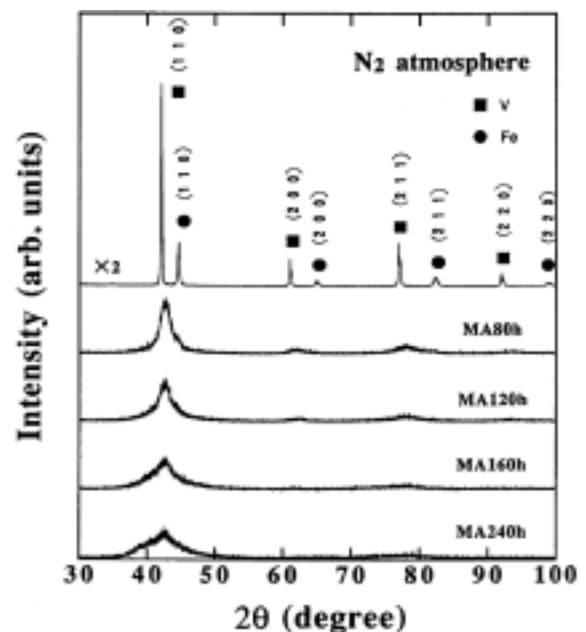
Fig. 1. The X-ray diffraction patterns for the \text{V}_{70}\text{Fe}_{30} powders subjected to mechanical alloying in \text{N}_2 gas atmosphere for different time intervals.
