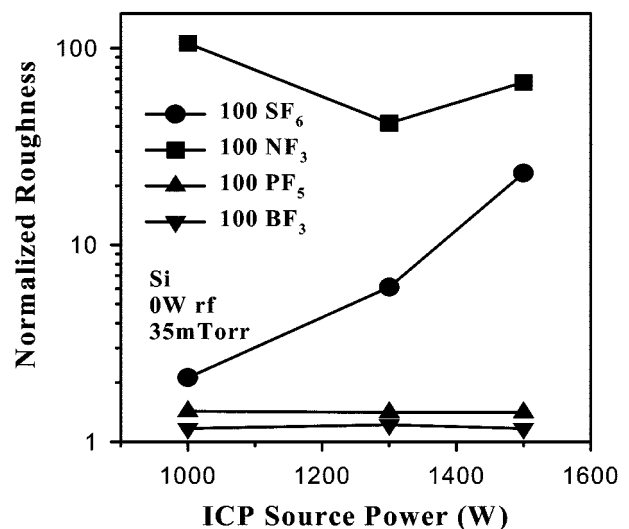
Fig. 7. RMS roughness of Si surfaces after etching in SF 6 , NF 3 , PF 5 , and BF 3 .
