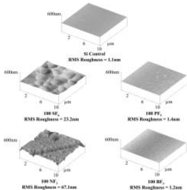
Fig. 6. AFM scans of Si surfaces before and after etching in SF 6 , NF 3 , PF 5 , and BF 3 .
