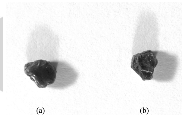
Fig. 1. A photograph of African rubies (a) non-treated and (b) heat-treated at 1500°C for 12 hrs in O 2 gas.
