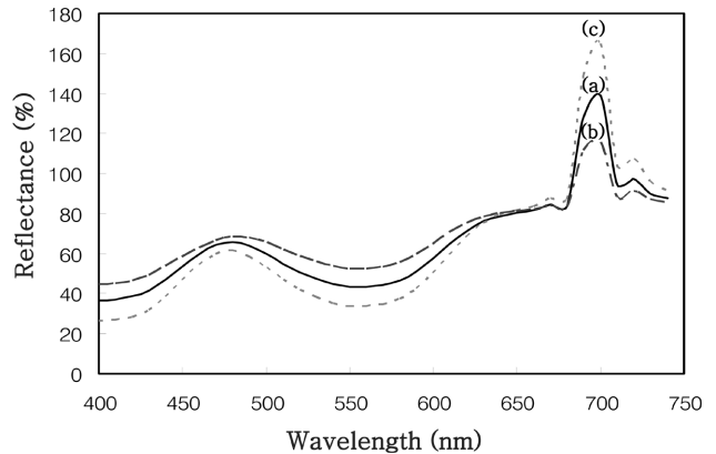
Fig. 4. Spectral reflectance graphs for African rubies (a) non-treated, (b) heat-treated at 1500°C for 12 hrs in O 2 gas and (c) hydrothermally treated at 450°C for 48 hrs in a Na 2 CO 3 -K 2 CO 3 solution.
