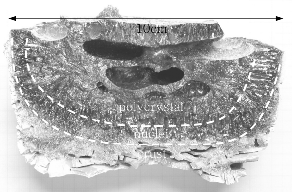
Fig. 7. Photograph of cross section of the ingot grown by uncontrolled cooling after keeping the melted condition for 9 hrs.
