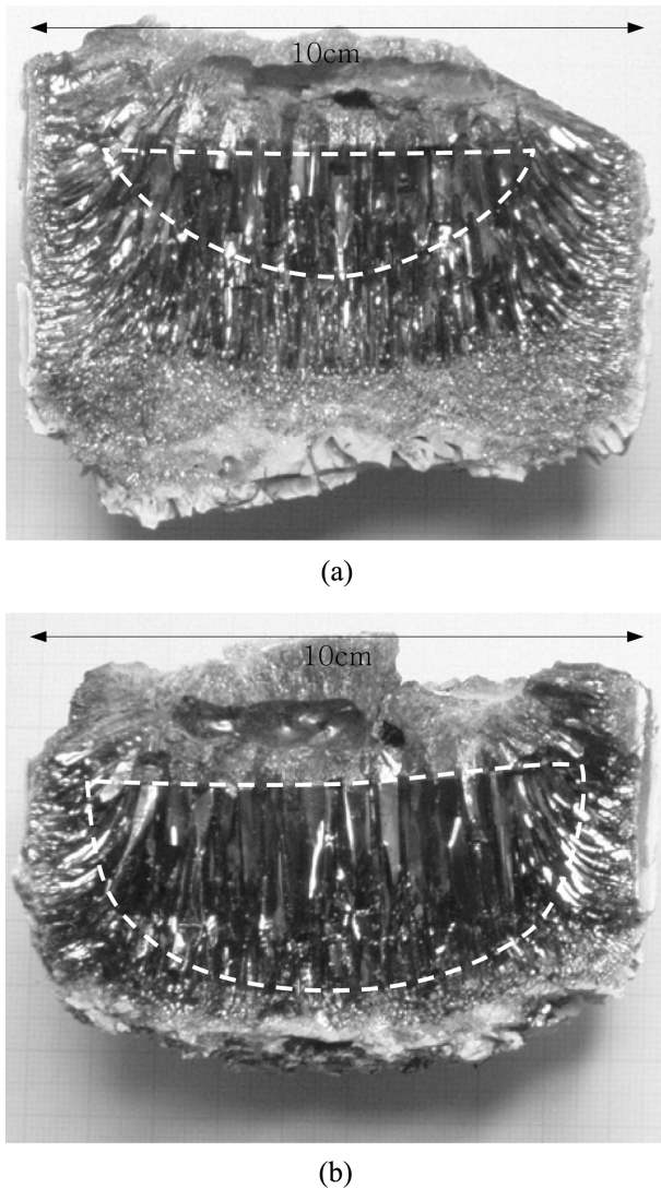
Fig. 8. Photographs of cross section of the ingots grown by controlled cooling after keeping the melted condition for 2 (a) and 9 hrs (b).
