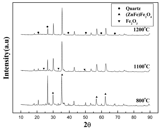
Fig. 9. XRD curves of 60 wt% EAF dust-40 wt% clay bodies with heat treatment temperature.
