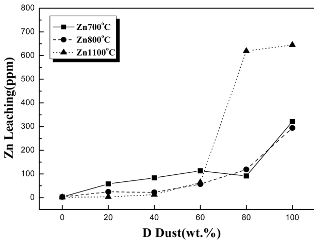
Fig. 6. TCLP leaching test results for zinc in the EAF dust-clay bodies.
