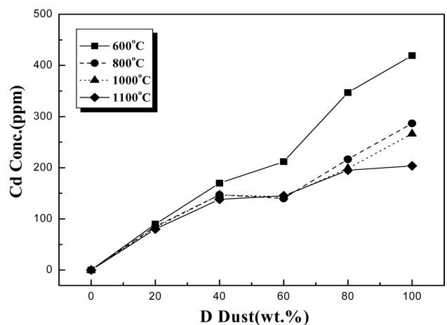
Fig. 1. Total concentration of cadmium in the EAF dust-clay bodies.
