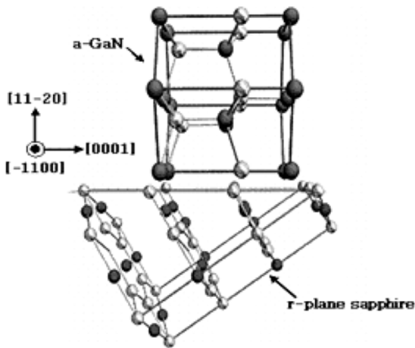
Fig. 2. Schematic image of a-plane GaN layer on r-plane sapphire substrate.
