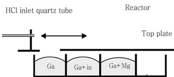
Fig. 1. The mixed-source HVPE with multi-sliding boat system.
