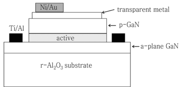
Fig. 4. The schematic structure of the SAG-GaN/InGaN heterostructure.
