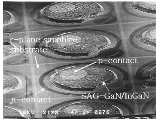
Fig. 5. Top-view image of SAG-GaN/InGaN heterostructure grown by the mixed-source HVPE with multi-sliding boat system.
