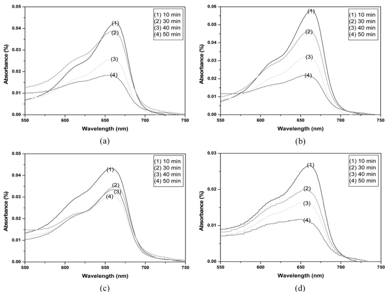
Fig. 5. UV/VIS spectra of MB concentration against the pitch coated \text{TiO}_2 under various time conditions; (a) PT64, (b) PT55, (c) PT46 and (d) PT37.
