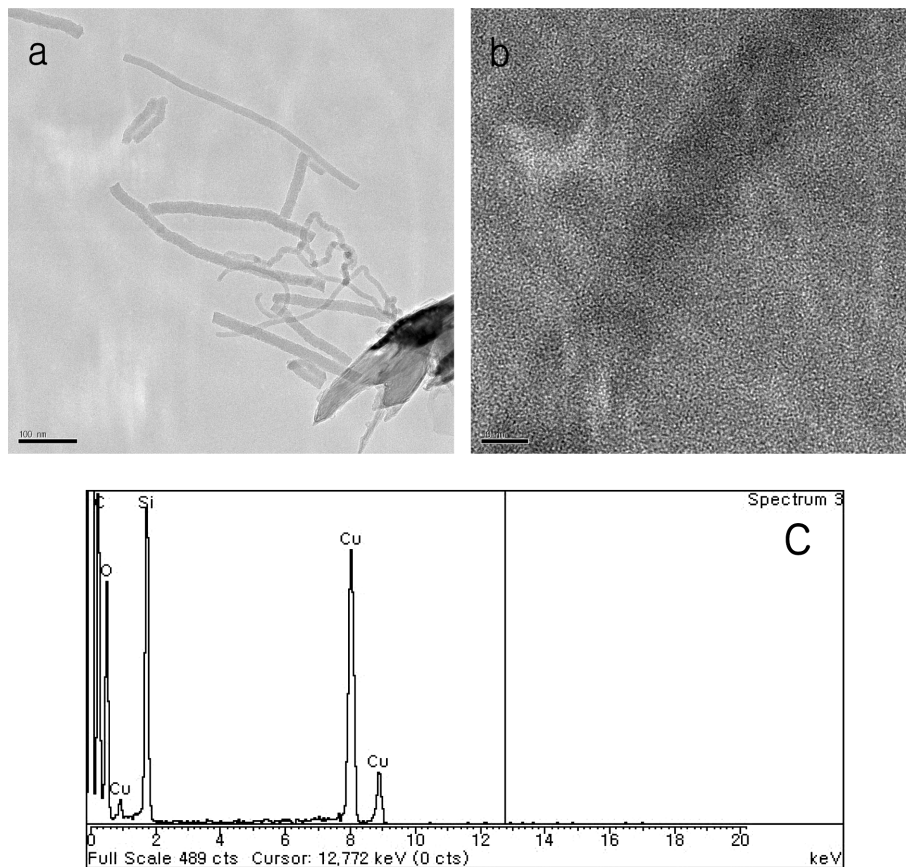
Fig. 3. TEM images of SiO x nanowires and EDX analysis (a) Low-magnification TEM image of SiO x , (b) HRTEM image of SiO x nanowire, (c) Chemical composition of SiO x nanowire.
