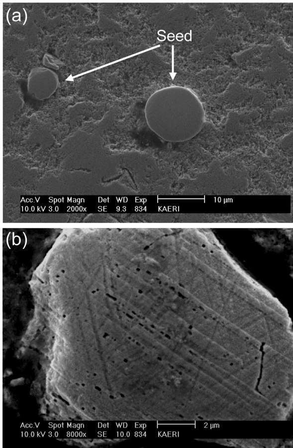
Fig. 5. Microstructures of 5 wt% seeded UO_2 compact heat-treated up to 1300^\circ C ; (a) the polished surface of a heat-treated compact and (b) the chemically-etched surface of a seed.
