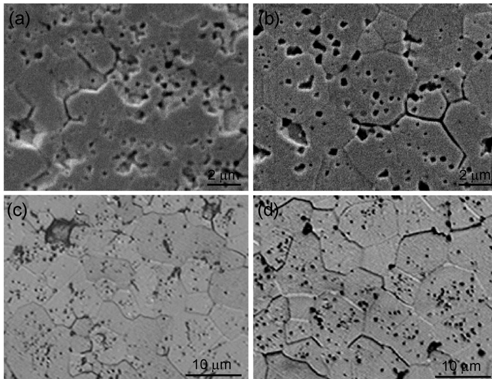
Fig. 3. Microstructures of ADU- UO_2 samples sintered at (a) 1600^\circ\text{C} for 0 h, (b) 1700^\circ\text{C} for 0 h, (c) 1700^\circ\text{C} for 1 h and (d) 1700^\circ\text{C} for 4 h.
