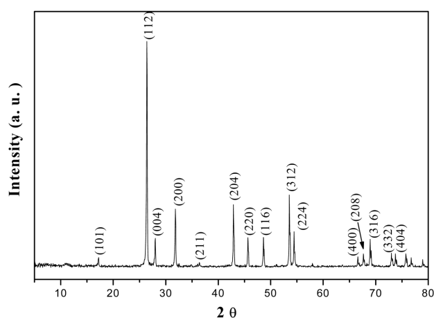
Fig. 3. XRD pattern and Miller indices of the as-synthesized BaWO 4 product.
