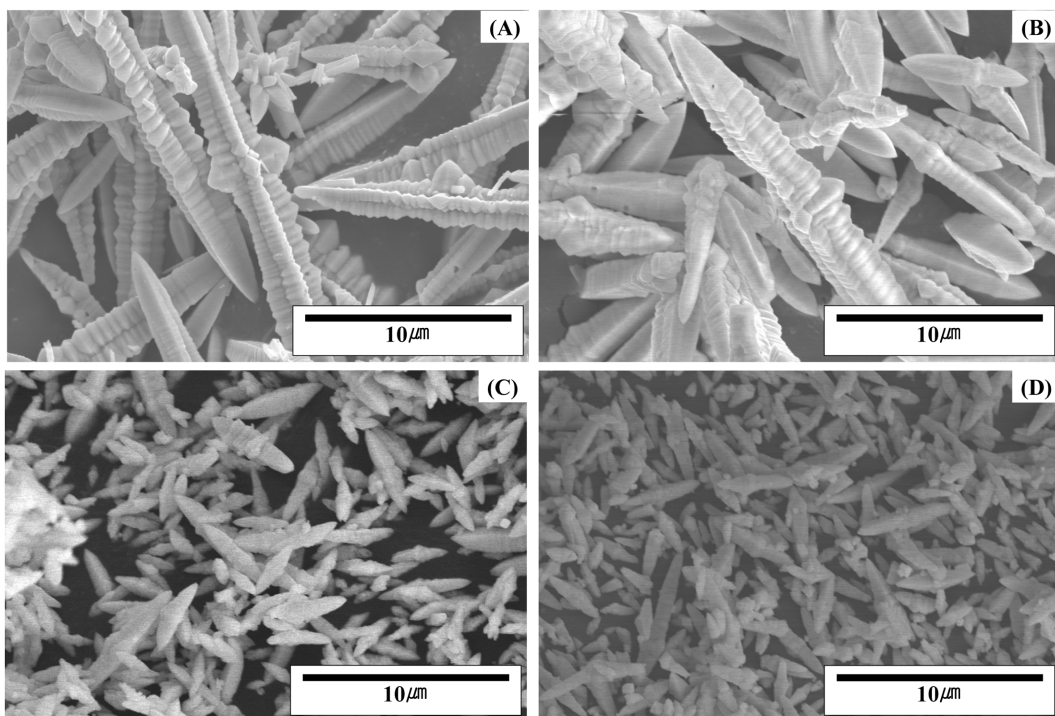
Fig. 6. SEM images of the as-synthesized BaWO_4 products obtained using different molar ratios of [WO_4^{2-}]/[Ba^{2+}] : (A) 0.5, (B) 1.0, (C) 2.0 and (D) 4.0.
