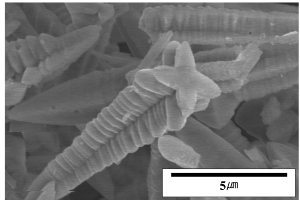
Fig. 5. SEM image of the as-synthesized BaWO_4 product obtained with 80 mM TMEDA.
