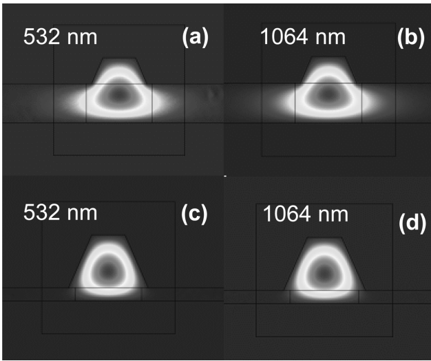
Fig. 4. Mode size simulation results of PPMgLN ridge-type waveguide at 532 and 1064 nm.
