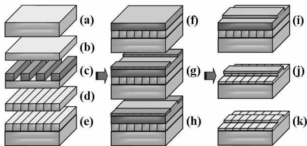
Fig. 1. QPM SHG device structure and fabrication sequence.
