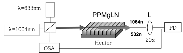
Fig. 5. Schematic of the experimental set-up used for SHG.
