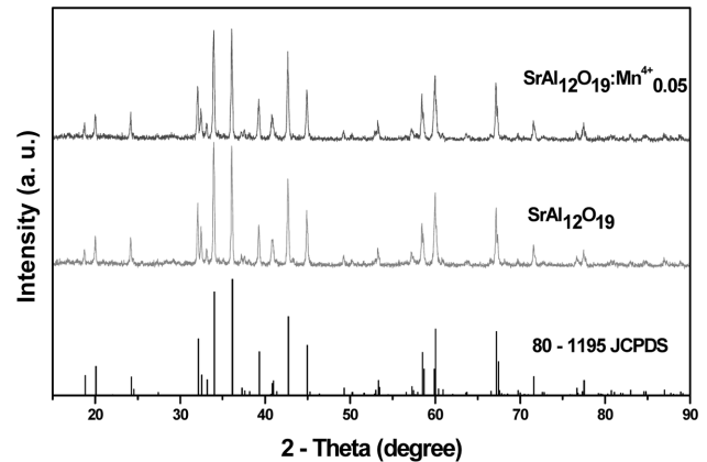
Fig. 1. X-ray diffraction pattern of \text{SrAl}_{12}\text{O}_{19} : \text{Mn}^{4+} powders sintered at 1500^\circ\text{C} for 6 hrs in air.
