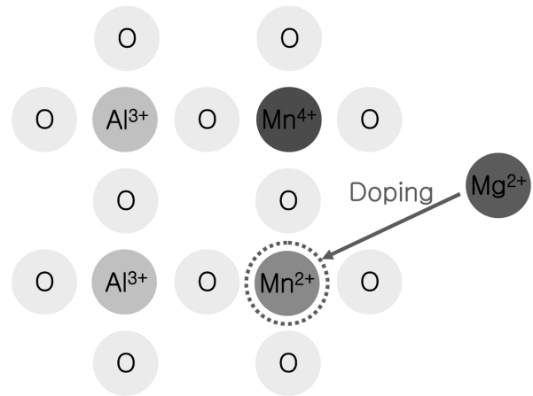
Fig. 4. Effect of Mg^{2+} charge compensation in SrAl_{12}O_{19}:Mn^{4+} .
