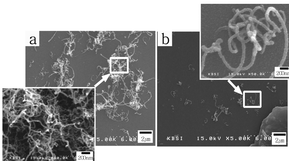
Fig. 5. FESEM images of as-deposited substrates at 850°C for (a) the sample with the cyclic modulation process, (b) the sample without the cyclic modulation process (Insets show the magnified images at the arrow position areas.).
