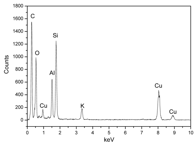
Fig. 3. TEM-EDX data of mica hydrothermally synthesized at 260°C for 72 hrs in a 8 mol% KOH solution.
