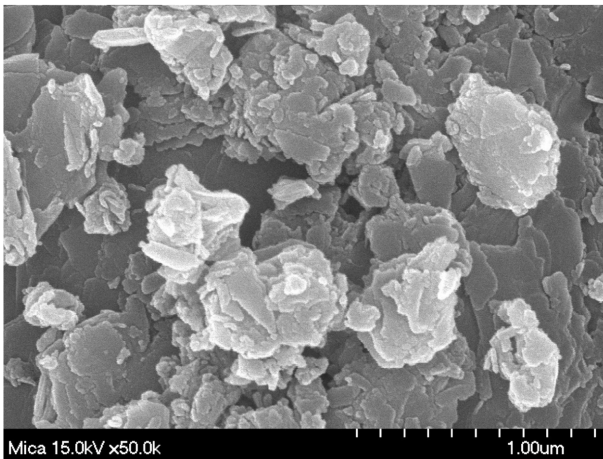
Fig. 4. SEM image of mica hydrothermally synthesized at 260°C for 72 hrs in a 8 mol% KOH solution.
