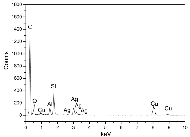
Fig. 13. TEM-EDX data of nano silver particle in the Fig. 12 area.
