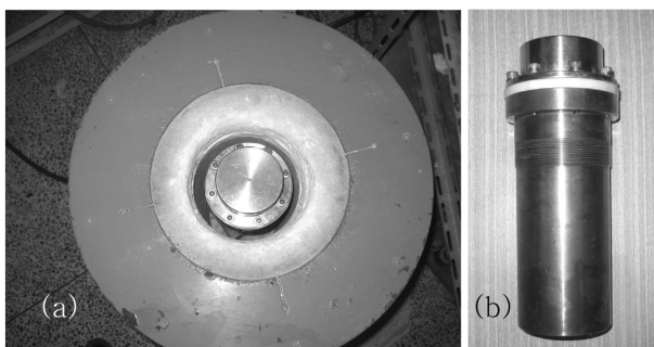
Fig. 5. Photographs of hydrothermal apparatus (a) and autoclave (b) for nano silver particle coating on the synthetic mica.
