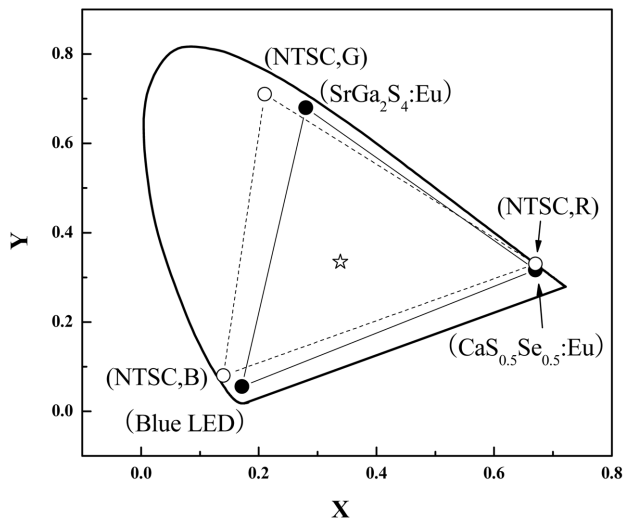
Fig. 10. CIE diagram and chromaticity coordinates of the blue LED, \text{SrGa}_2\text{S}_4 :Eu, and \text{CaS}_{0.50}\text{Se}_{0.50} :Eu, as well as NTSC blue, NTSC green, and NTSC red. ☆ represents the chromaticity coordinates of the three-band white LED fabricated by doping \text{SrGa}_2\text{S}_4 :Eu and \text{CaS}_{0.50}\text{Se}_{0.50} :Eu phosphors onto a blue LED chip.
