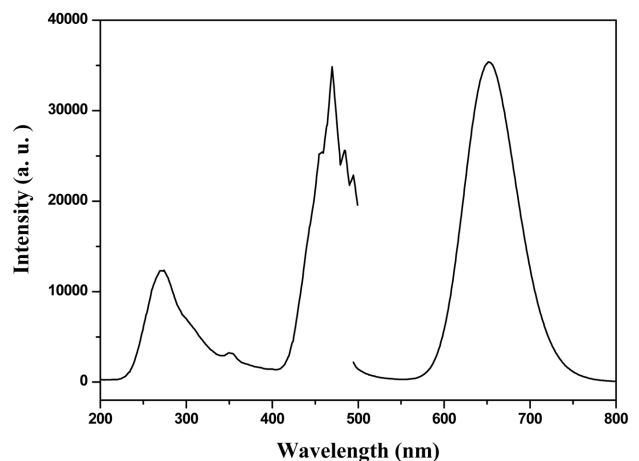
Fig. 1. Photoluminescence excitation and emission spectra of \text{CaS} :Eu phosphor.
