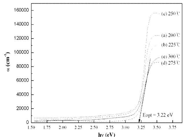
Fig. 6. Absorption coefficient versus h\nu plot from the results related to transmittance spectra. Preheated at (a) 200°C (b) 225°C (c) 250°C (d) 275°C (e) 300°C.
