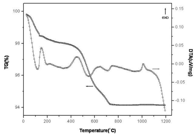
Fig. 6. TG-DTA curves of raw material (RO).
