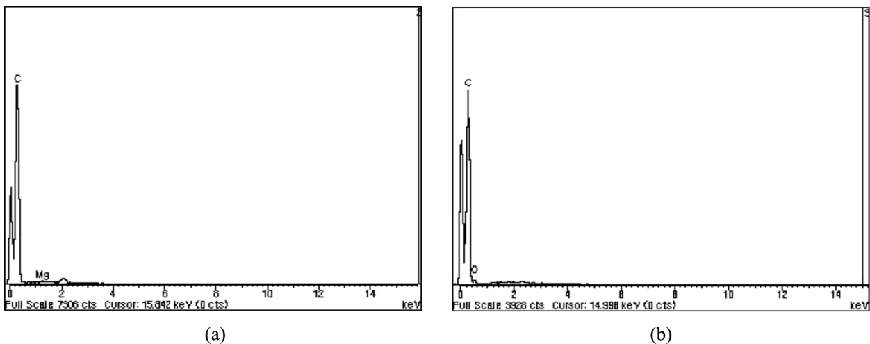
Fig. 4. EDS analysis of (a) as-received and (b) bead milled M-CNTs.
