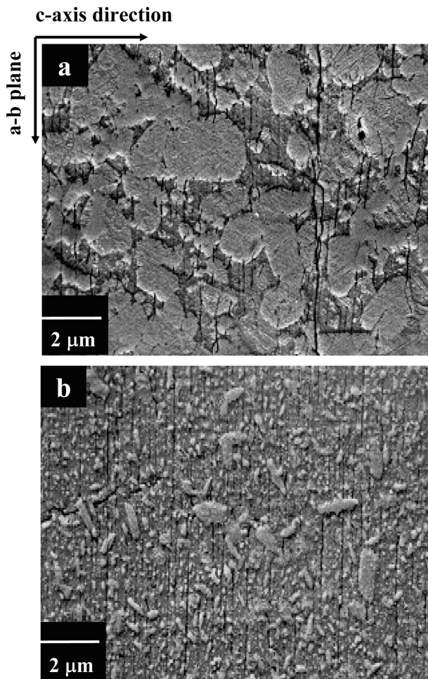
Fig. 4. SEM micrographs of the directionally melt-textured (a) (YNS)-123 and (b) (YNS)-123 crystal with 1 wt% CeO 2 additions. Note finely dispersed (YNS)211 inclusions are trapped into the (YNS)123 matrix with platelet crystals.
