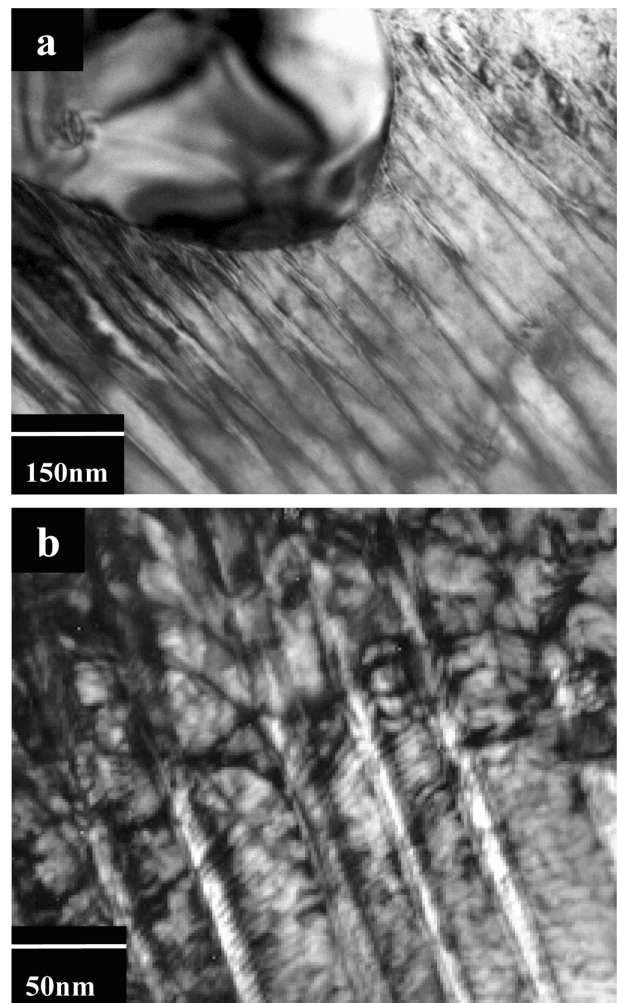
Fig. 5. TEM micrograph of the directionally melt-textured (YNS)-123 crystal with 1 wt% CeO 2 additive. The (YNS)211 inclusion, dense twin patterns, dislocations and nano-sized defects are seen in the image.
