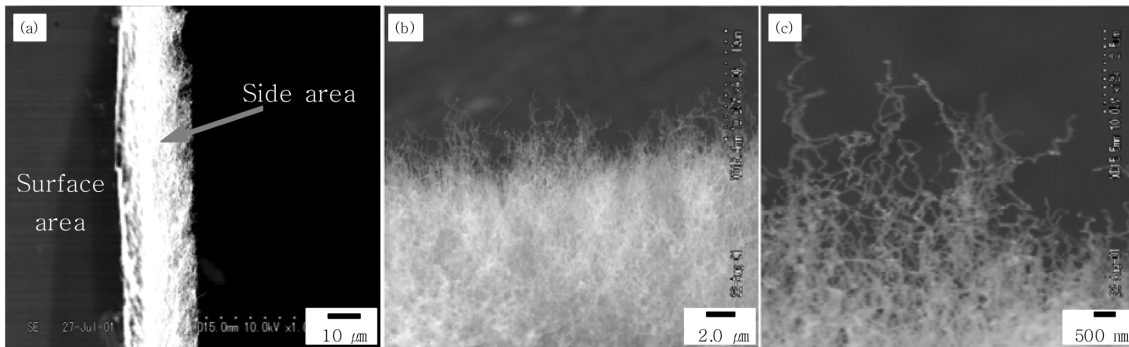
Fig. 3. (a) FESEM image of the carbon nanofilaments on the surface and the side area of the substrate under the remote plasma condition. (b) The magnified FESEM image of Fig. 3a and (c) the magnified FESEM image of Fig. 3b.
