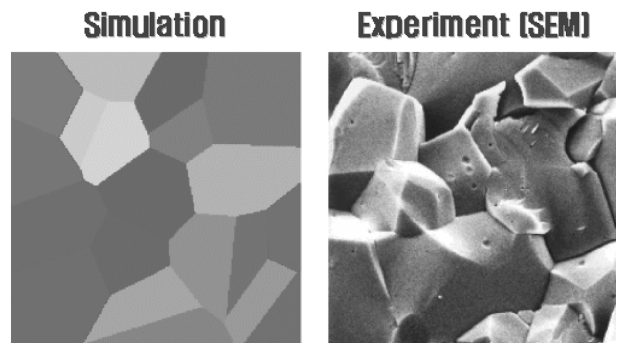
Fig. 8. Comparison of grain growth of Al_2O_3 in sintering temperature 1650^\circ C between simulation and experiment.
