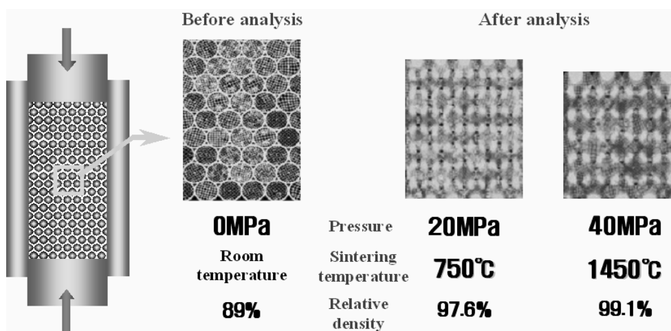
Fig. 4. Relative density in sintering temperature 1450°C and holding pressure 40 MPa.
