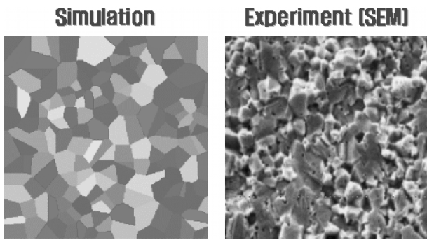
Fig. 7. Comparison of grain growth of Al_2O_3 in sintering temperature 1450^\circ C between simulation and experiment.
