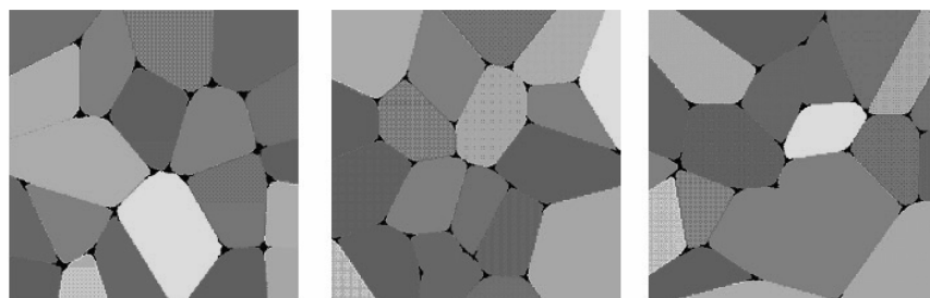
Fig. 9. Monte Carlo Simulation for getting grain growth and relative density in sintering temperature 1450^\circ C .
