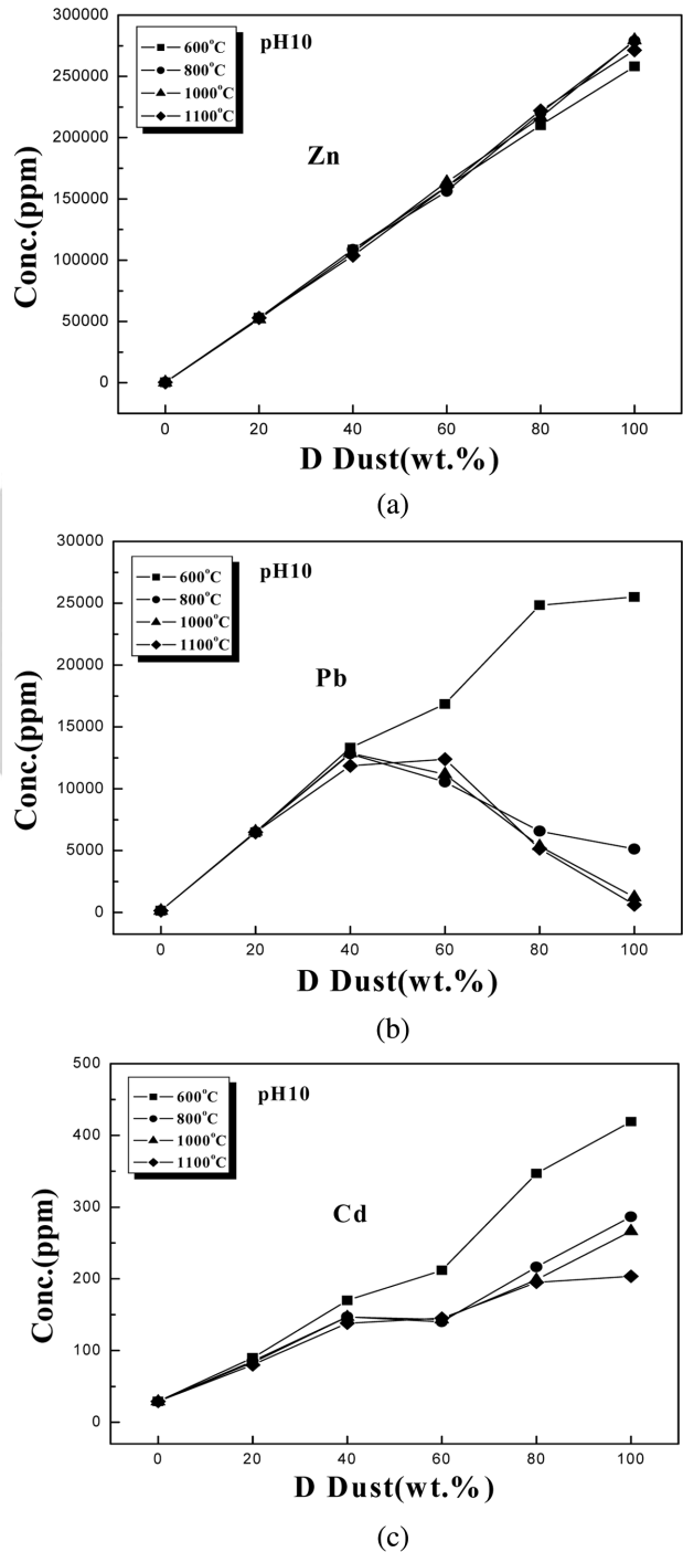
Fig. 3. Total quantity of heavy metals ((a) Zn, (b) Pb, (c) Cd) in EAF dust-clay bodies with various sintering temperature and mixing ratios.
