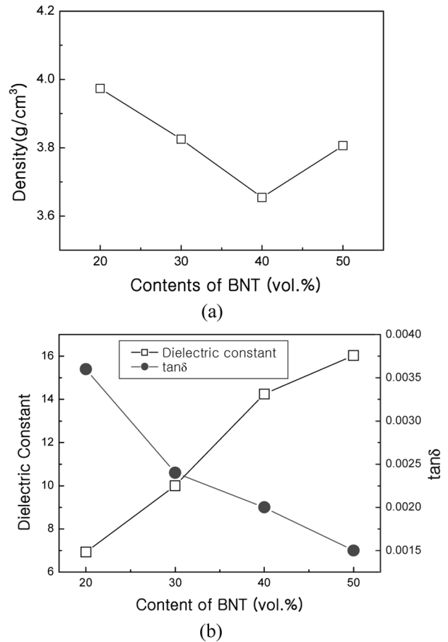
Fig. 7. Density (a) and dielectric properties (b) of BCB/BNT composite cured at 250°C as a function of BNT content.
