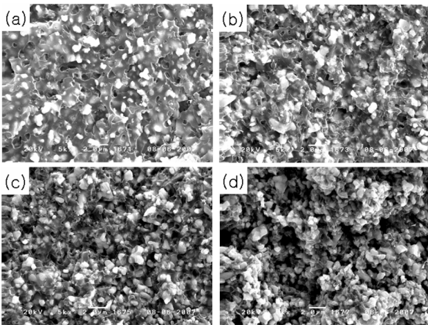
Fig. 8. SEM images of BCB/BNT composite with BNT contents (a) 20 vol%, (b) 30 vol%, (c) 40 vol%, and (d) 50 vol%.
