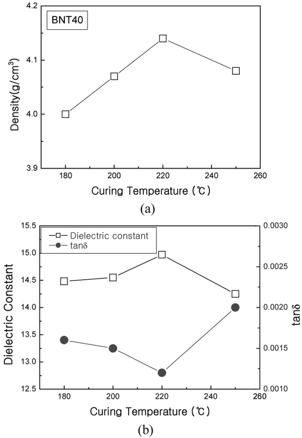
Fig. 6. Density (a) and dielectric properties (b) of BCB/BNT composite (BNT40) as a function of curing temperature.
