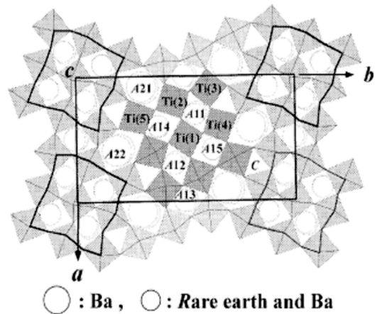
Fig. 2. Schematic diagram of Tungsten-bronze structure of BNT.
