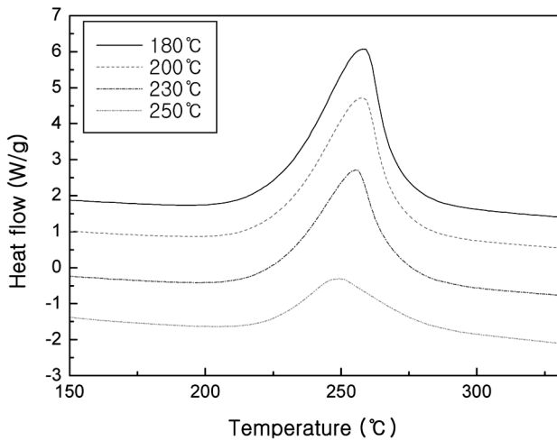
Fig. 3. DSC curves of BCB/BNT composite (BNT40) as a function of temperature.
