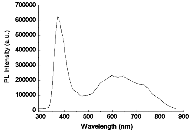
Fig. 4. Photoluminescence spectrum of GaN nanowires measured at room temperature.
