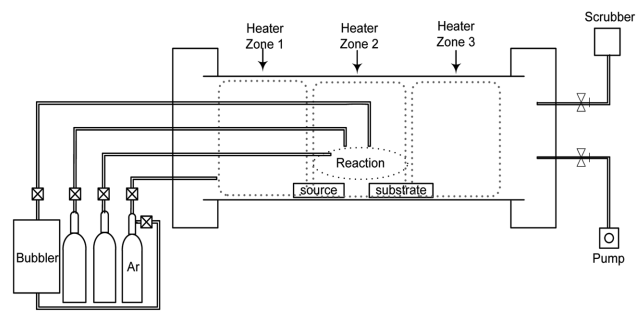
Fig. 1. A schematic diagram of GaN nanowires synthesis equipment.
