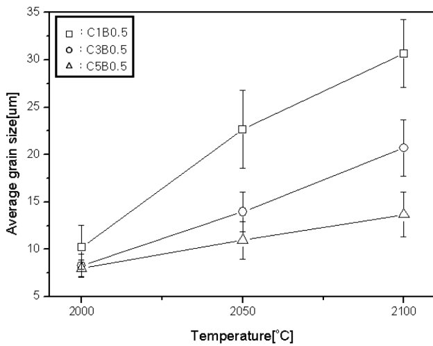
Fig. 6. The effect of sintering temperature and carbon content on average grain size of SiC specimens.
