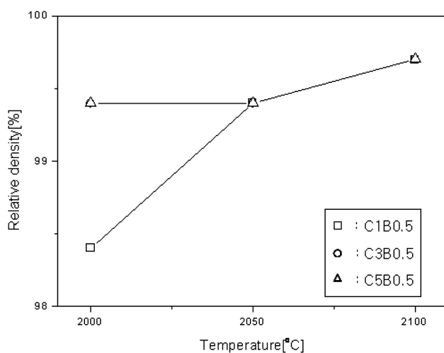
Fig. 2. The effect of sintering temperature and carbon content on the apparent relative density of SiC specimens.
