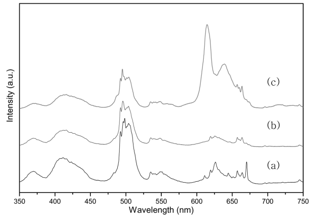
Fig. 5. Photoluminescence spectra of \text{CaZrO}_3 : \text{Li}, \text{Pr} at 1400^\circ\text{C} in \text{N}_2 gas; (a) \text{B}_2\text{O}_3 1 mol%, (b) 5 mol%, (c) 10 mol%.
