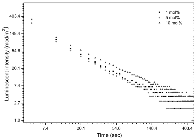
Fig. 8. Luminescence-time characteristics of as-grown CaZrO 3 :Li, Pr phosphors.
