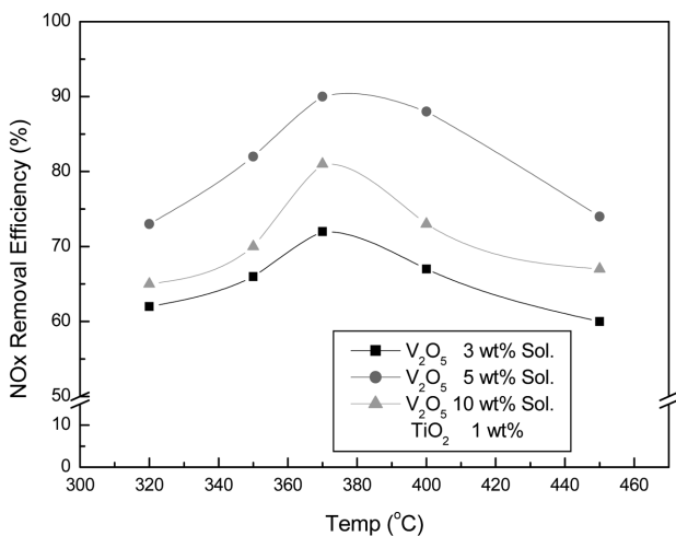
Fig. 4. NO x removal efficiency with variation of V 2 O 5 concentration and temperature.
