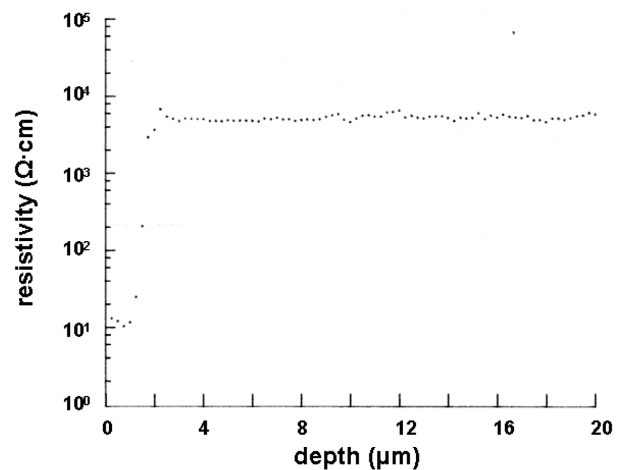
Fig. 2. The resistivity depth profile of the wafer with 16 ppma oxygen concentration after 3 step and donor formation.
