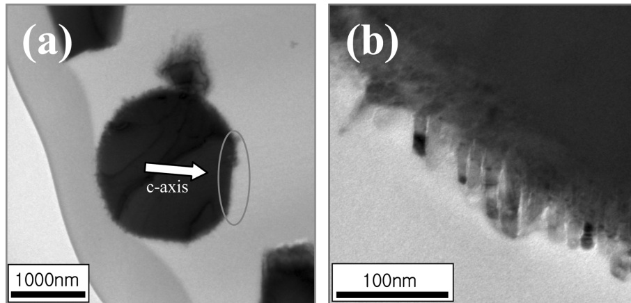
Fig. 2. BF-TEM images of as-grown sample at the interface between Zn and ZnO (a) Low-magnification and (b) High-magnification.
