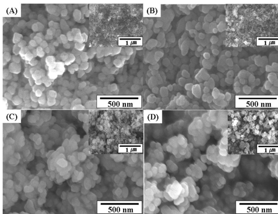
Fig. 7. SEM images of the \text{CaMoO}_4 crystals synthesized by microemulsion method with [\text{Ca}^{2+}] = [\text{WO}_4^{2-}] = 0.5 \text{ M} for various values of w : (A) 5, (B) 10, (C) 15, and (D) 20.
