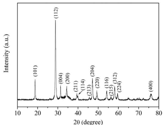
Fig. 1. XRD pattern and Miller indices of CaMoO 4 product synthesized by precipitation method at room temperature with [Ca 2+ ] = [MoO 4 2- ] = 0.5 M.
