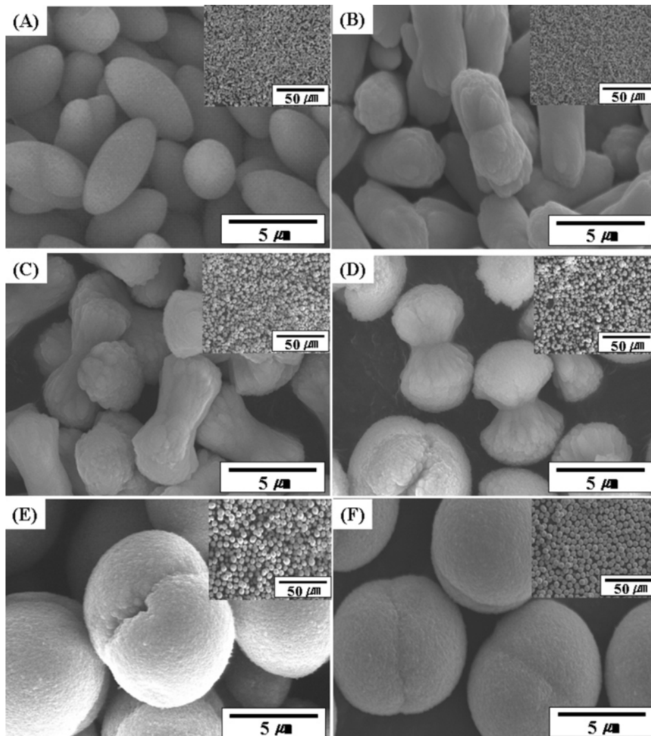
Fig. 3. SEM images of the \text{CaMoO}_4 crystals synthesized by precipitation method at room temperature with various concentrations of [\text{Ca}^{2+}] = [\text{WO}_4^{2-}] : (A) 0.05 M, (B) 0.1 M, (C) 0.2 M, (D) 0.3 M, (E) 0.4 M, and (F) 0.5 M. The insets show SEM images of the \text{CaMoO}_4 crystals with different magnifications.
