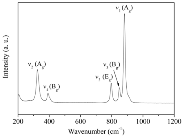
Fig. 2. Raman spectrum of \text{CaMoO}_4 product synthesized by precipitation method at room temperature with [\text{Ca}^{2+}] = [\text{MoO}_4^{2-}] = 0.5 \text{ M} .
