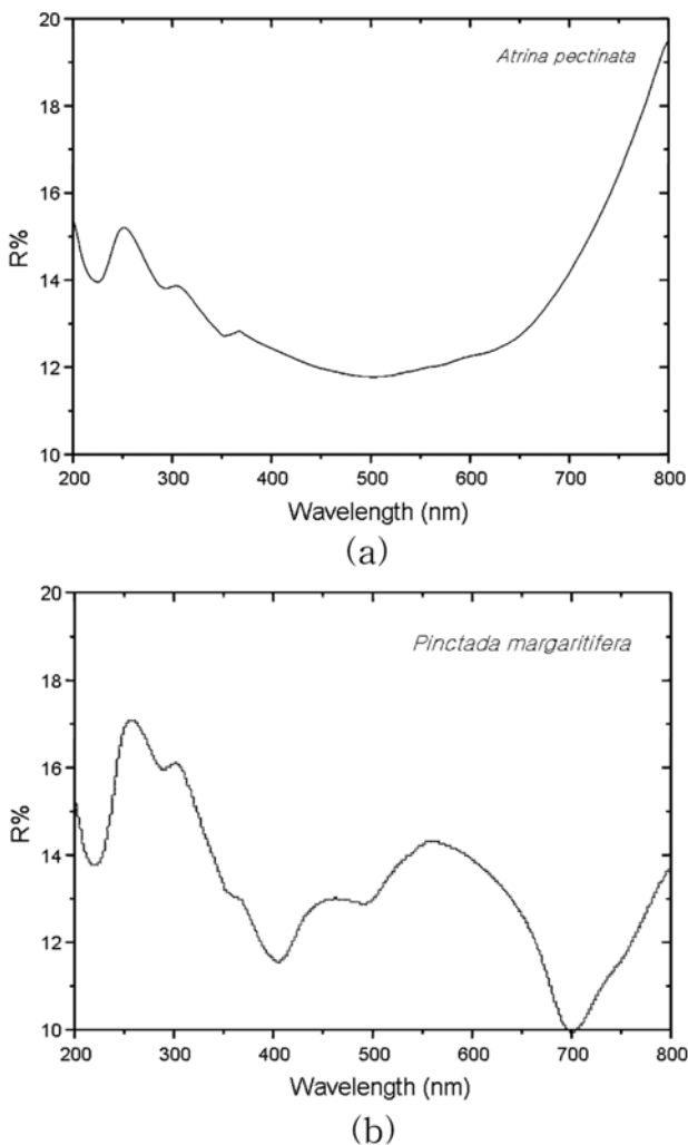
Fig. 4. UV-Vis spectra of pearls cultured using the (a) Atrina pectinata and (b) P. margaritifera .
