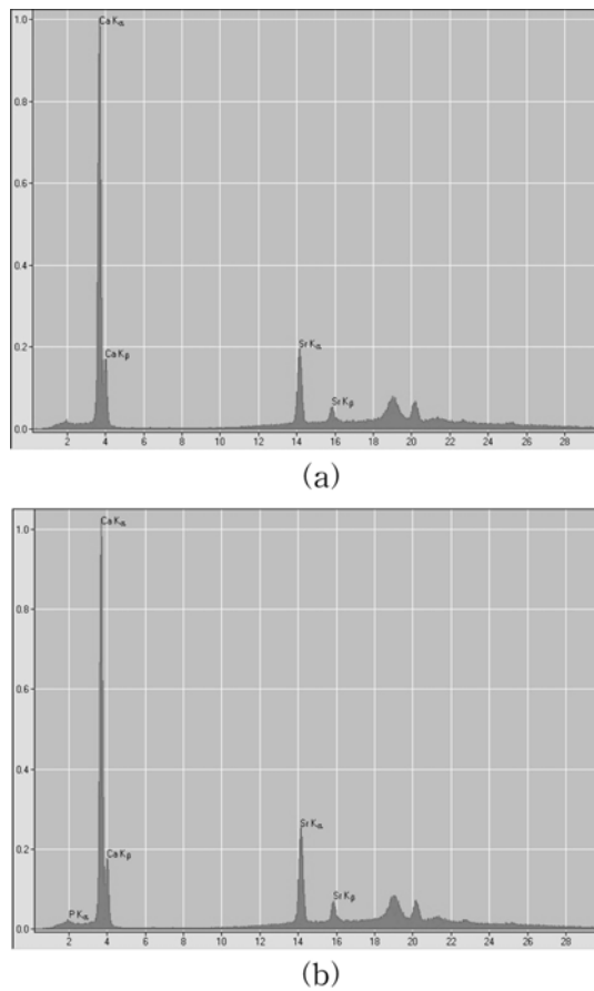
Fig. 5. XRF spectra of (a) Atrina pectinata pearl and (b) P. margaritifera pearl.
