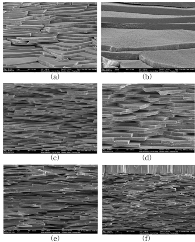
Fig. 3. FE-SEM micrographs of fracture surfaces of nacre (a), (b); Atrina pectinata pearl (c), (d); P. margaritifera pearl and (e), (f); inner surface of Atrina pectinata shell. (f) image shows calcite structure (upper region of image) contact with aragonite tablets.
