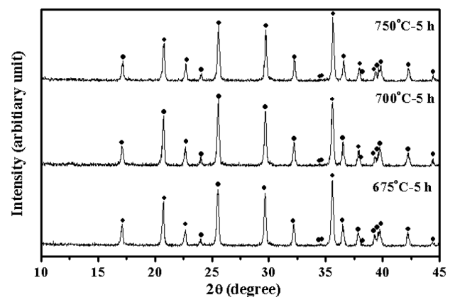
Fig. 2. XRD patterns of LiFe 0.965 Cr 0.03 Al 0.005 PO 4 powders heat treated at 675~750°C for 5 h.
