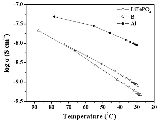
Fig. 7. Electrical conductivities of \text{LiFePO}_4 , \text{LiFe}_{0.965}\text{Cr}_{0.035}\text{B}_{0.005}\text{PO}_4 and \text{LiFe}_{0.965}\text{Cr}_{0.035}\text{Al}_{0.005}\text{PO}_4 powders heat treated at 675^\circ\text{C} for 5 h.
