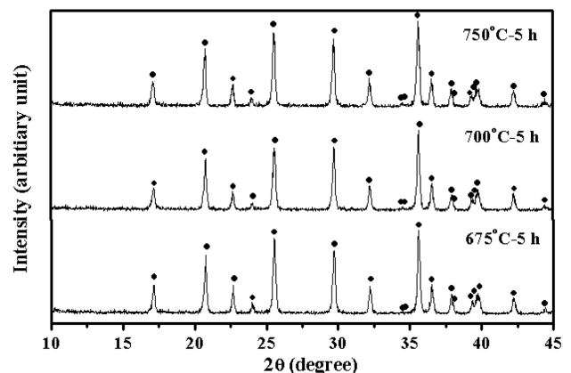
Fig. 1. XRD patterns of LiFe 0.965 Cr 0.03 B 0.005 PO 4 powders heat treated at 675~750°C for 5 h.
