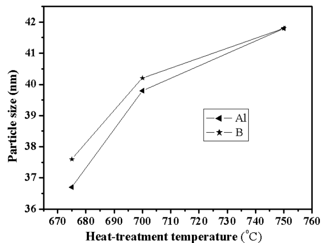
Fig. 6. Estimated particle sizes of LiFe 0.965 Cr 0.03 B 0.005 PO 4 and LiFe 0.965 Cr 0.03 Al 0.005 PO 4 powders at the heat treated temperatures using Scherrer equation ( t = 0.9 \cdot \lambda / (B \cos \theta)^{-1} ; t = particle size, \lambda = wave length, B = FWHM (radian), \theta = diffraction angle (degrees)).
