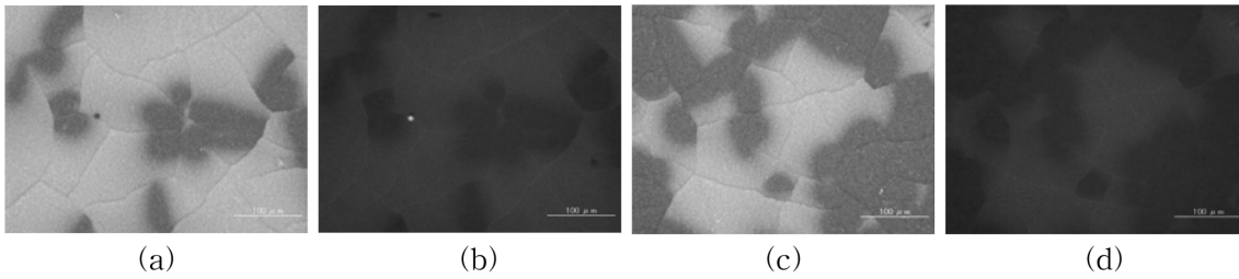
Fig. 1. Optical images of GaN layer by process II; (a) GaN/CoSi 2 /Si(100), (b) GaN/CoSi 2 /Si(100) in UV mode, (c) GaN/CoSi 2 /Si(111), and (d) GaN/CoSi 2 /Si(111) in UV mode.
