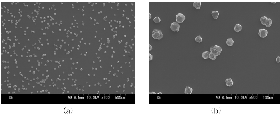
Fig. 2. FESEM image of GaN layer after process I; (a) × 100 observation and (b) × 500 observation.
